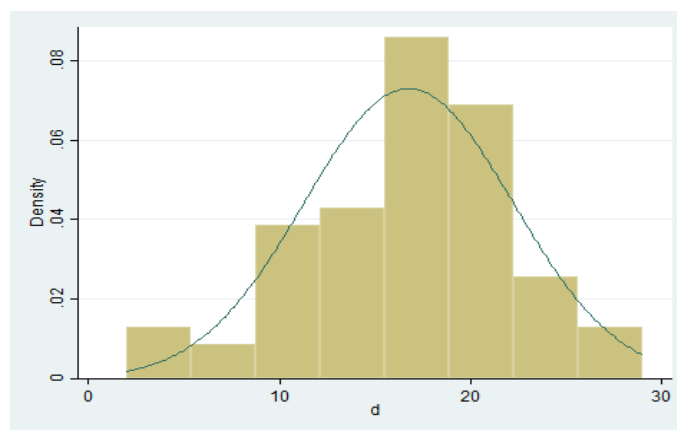
Figure 2. Independent variables distribution
